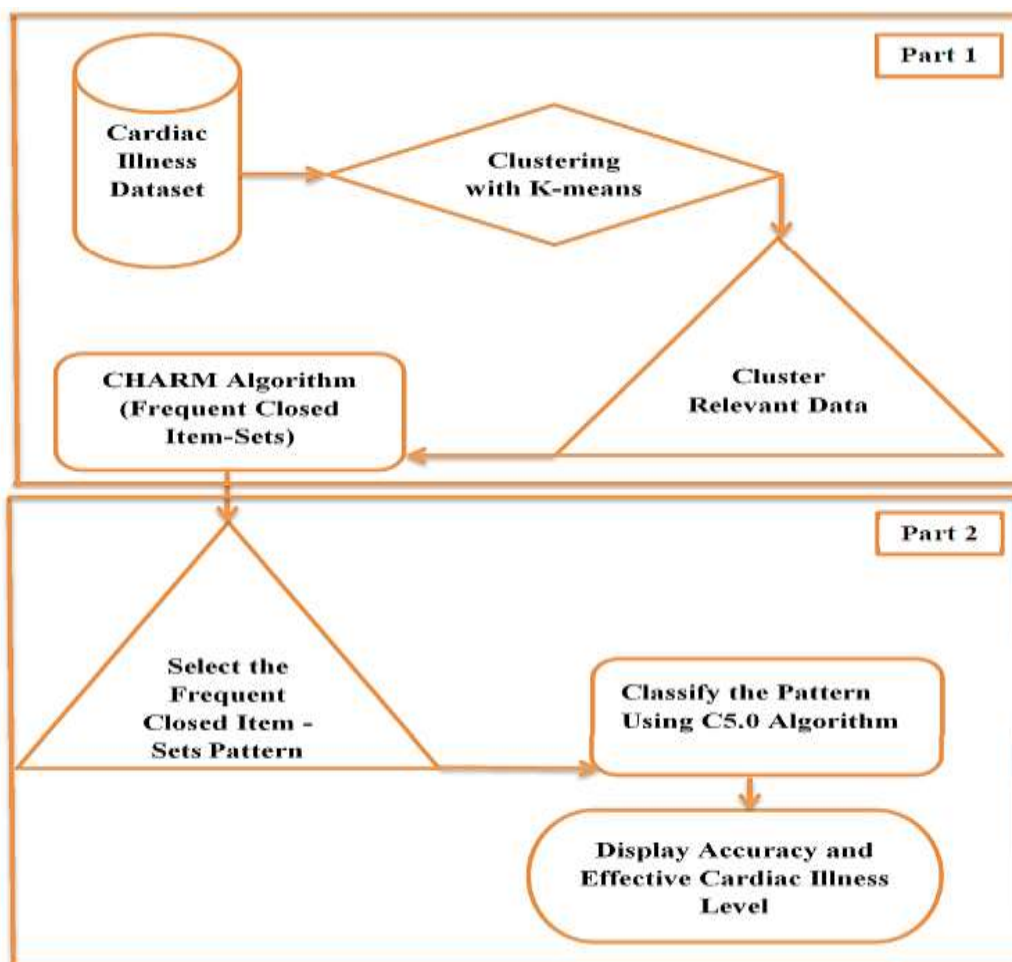
Figure 2. The Proposed System Architecture Steps
